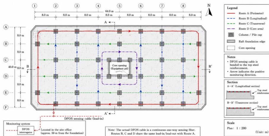
Figure 3. Layout of the DFOS sensing route in the raft foundation slab
