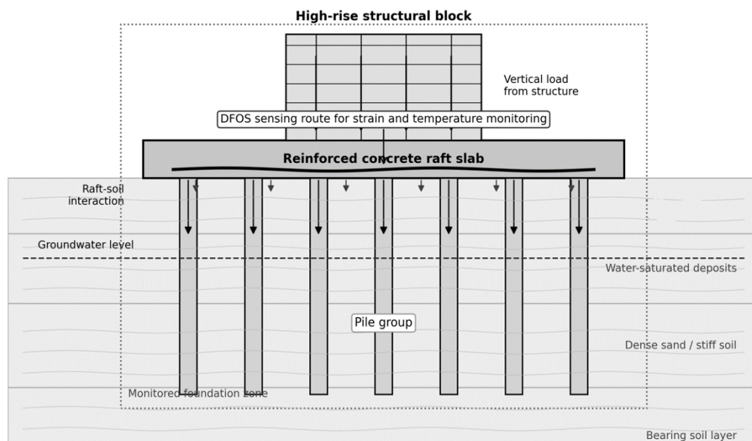
Figure 2. Conceptual scheme of the pile-raft foundation system and load transfer mechanism Note – adapted by the authors based on engineering-geological survey materials
