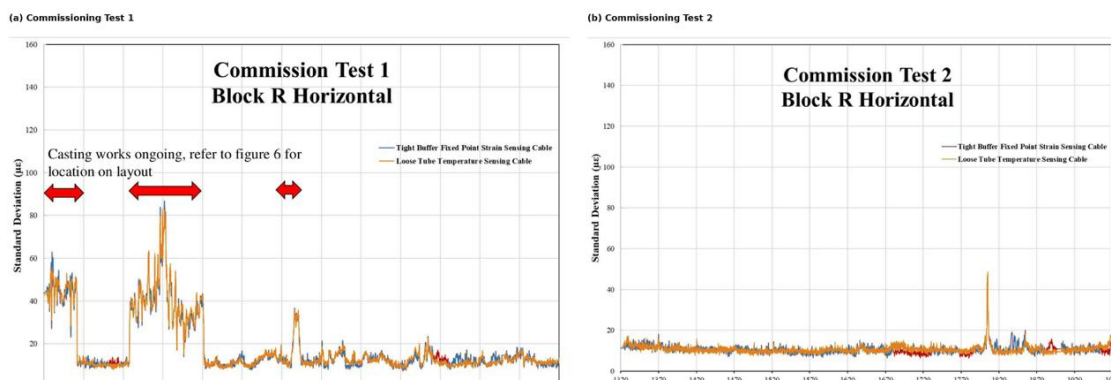
Figure 5. Comparison of distributed standard deviation profiles obtained during the first and second commissioning tests along the Block R horizontal sensing route
