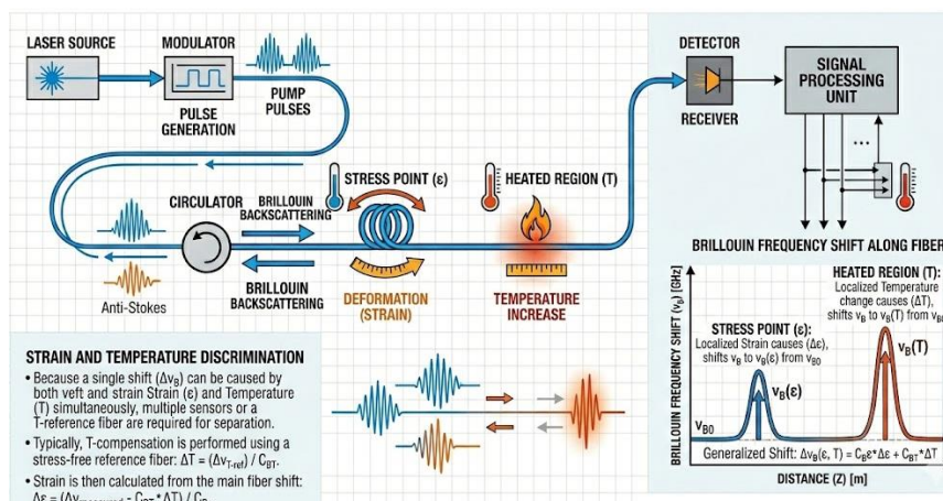
Figure 4. Principle of BOTDA-based distributed strain and temperature measurement
