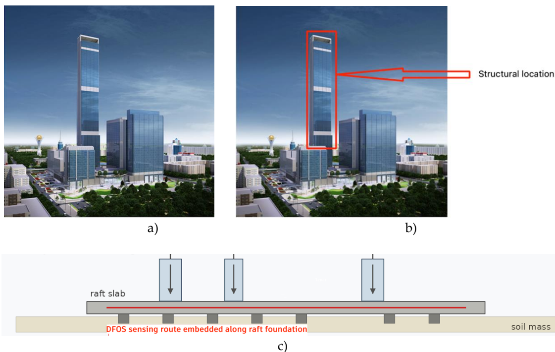
Figure 1. General view and structural location of Block R in the Abu Dhabi Plaza high-rise building complex: a) general view; b) structural location; c) simplified monitoring concept at foundation level
